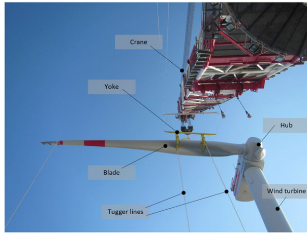
FIGURE 1 Illustration of the mating phase during a single blade installation. (Image source: RWE GmbH 28 ) [Colour figure can be viewed at wileyonlinelibrary.com]
